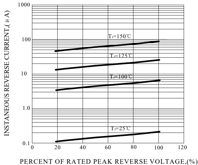
FIG.5-TYPICAL REVERSE CHARACTERISTICS
